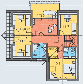
POSCHODIE [plocha 96.5 m 2 ]
