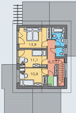
POSCHODIE [plocha 50.7 m 2 ]
