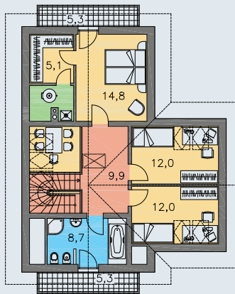
POSCHODIE [plocha 76.5 m 2 ]
