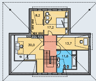
POSCHODIE [plocha 87.0 m 2 ]
