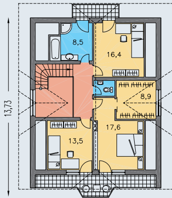
POSCHODIE [plocha 84.6 m 2 ]
