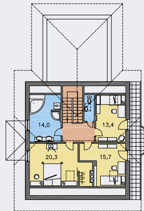
POSCHODIE [plocha 94.8 m 2 ]
