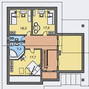
POSCHODIE [plocha 75.5 m 2 ]
