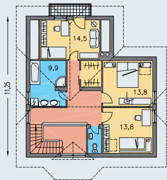
POSCHODIE [plocha 74.4 m 2 ]
