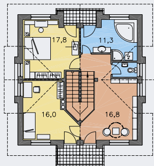
POSCHODIE [plocha 76.6 m 2 ]
