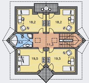
POSCHODIE [plocha 105.7 m 2 ]
