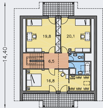
POSCHODIE [plocha 97.7 m 2 ]
