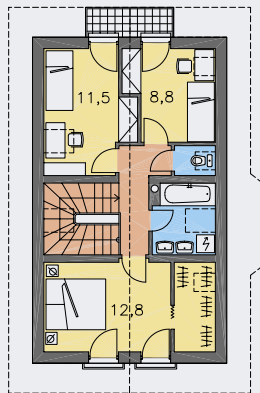
POSCHODIE [plocha 50.9 m 2 ]
