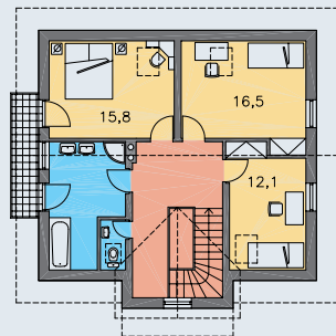
POSCHODIE [plocha 73.4 m 2 ]
