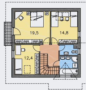
POSCHODIE [plocha 63.8 m 2 ]
