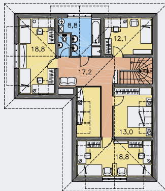
POSCHODIE [plocha 90.4 m 2 ]
