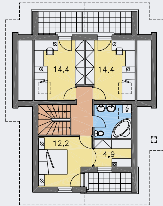
POSCHODIE [plocha 71.7 m 2 ]
