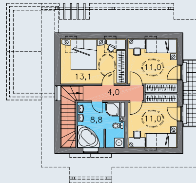
POSCHODIE [plocha 52.4 m 2 ]
