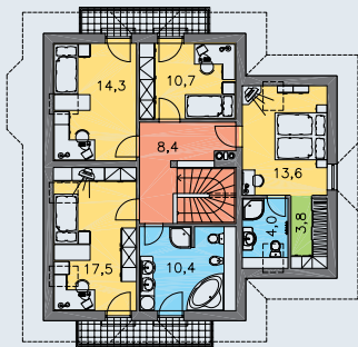
POSCHODIE [plocha 93.0 m 2 ]
