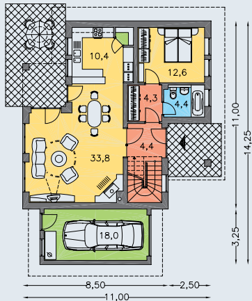
POSCHODIE [plocha 95.6 m 2 ]
