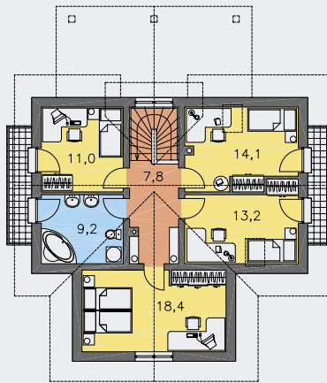
POSCHODIE [plocha 83.3 m 2 ]
