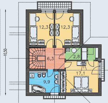
POSCHODIE [plocha 67.8 m 2 ]
