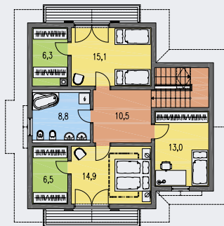
POSCHODIE [plocha 86.3 m 2 ]
