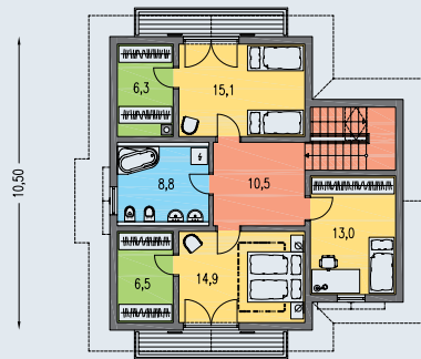
POSCHODIE [plocha 86.3 m 2 ]
